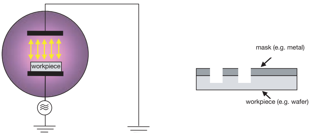
fig. 150: RIE operation
