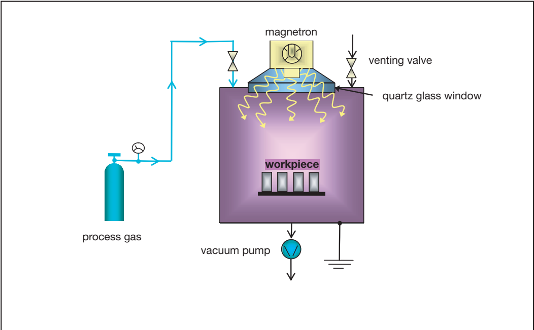
fig. 2: schematic of a microwave plasma system (2,45 GHz) with metal chamber
