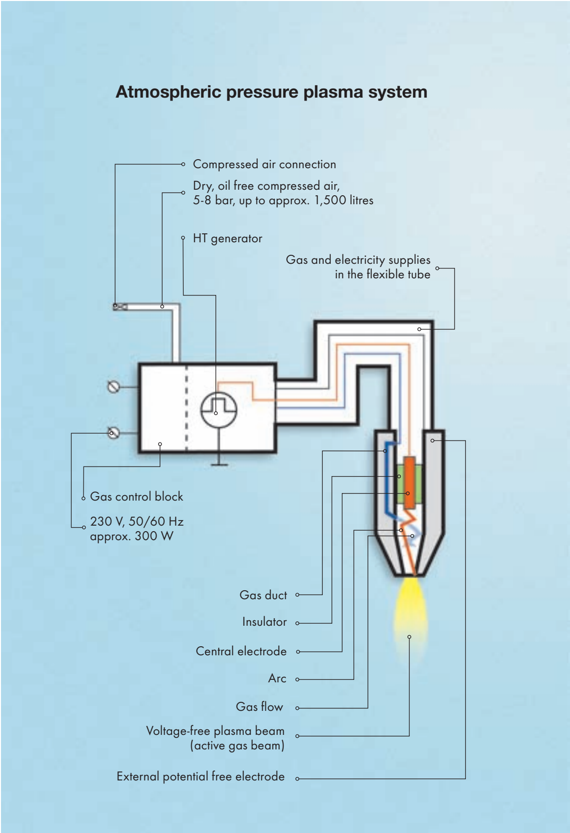
fig. 168: functional principle of a atmospheric plasma system
