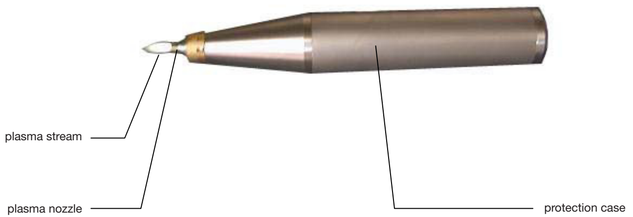
fig. 172: plasma device
